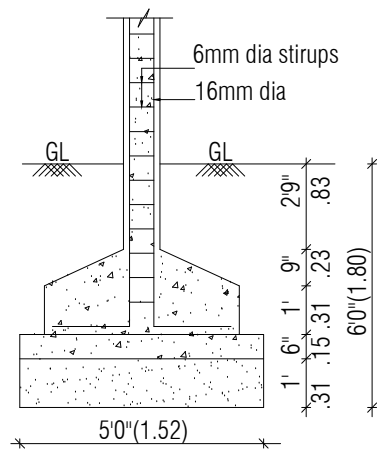
FOUNDATION DETAIL
