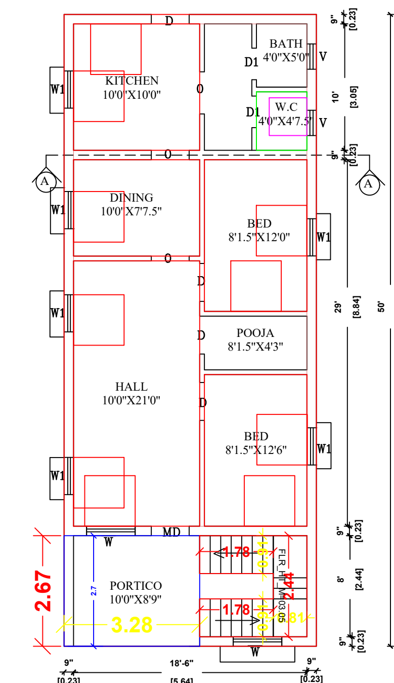
GROUND FLOOR PLAN (BLOCK-2)
