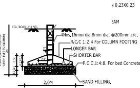
FOUNDATION DETAIL
