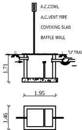
SEPTIC TANK
