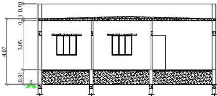
SECTION "SC"
