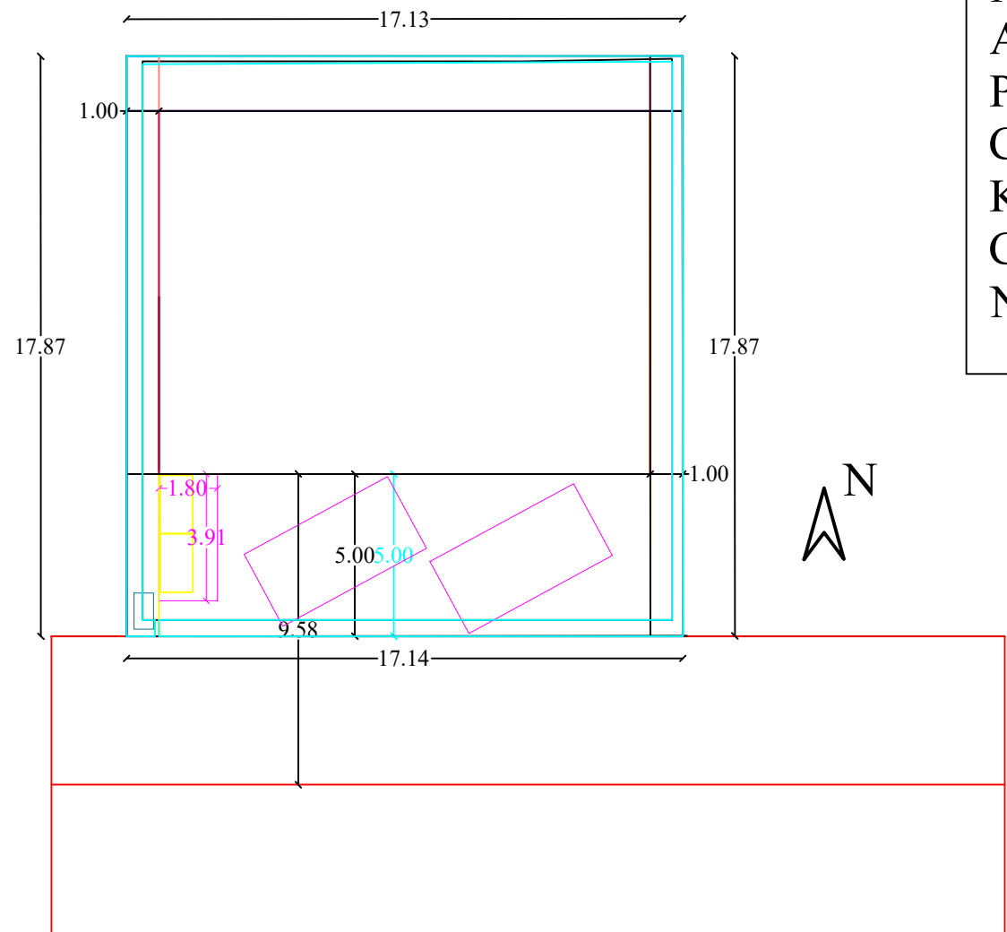
SITE PLAN
