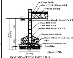
FOUNDATION DETAILS (Scale 1:50)
