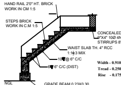
STAIRCASE DETAILS (Scale 1:50)
