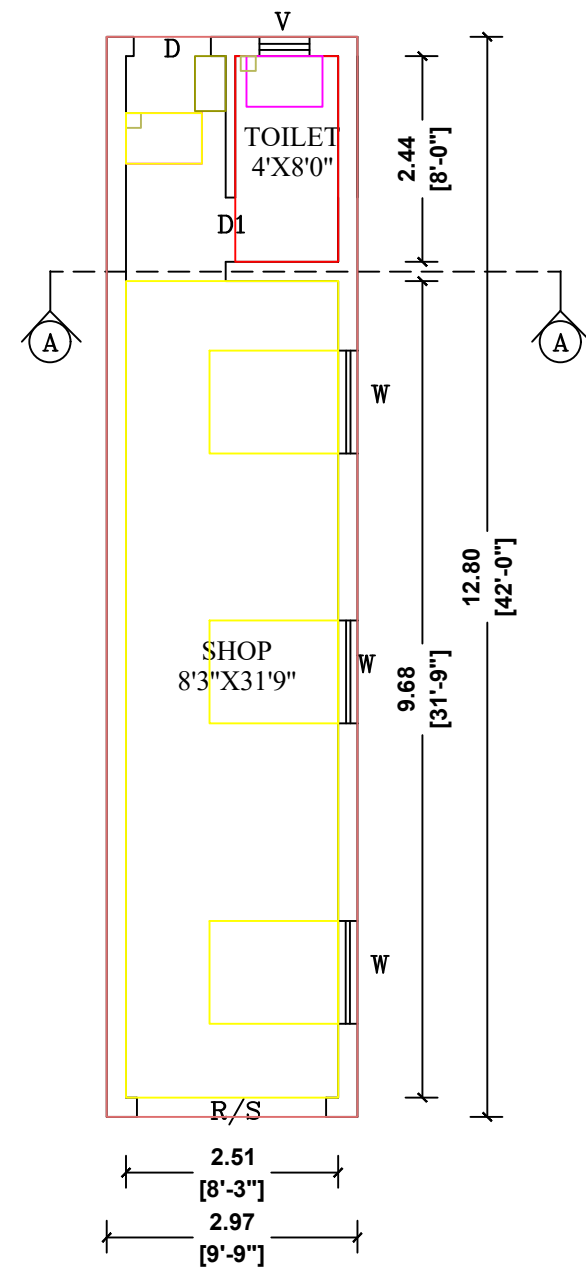
PROPOSED PLAN
