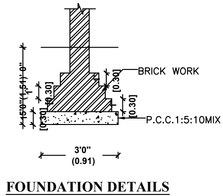
FOUNDATION DETAILS
