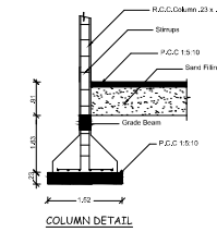
COLUMN DETAIL
