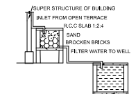
RAINWATER HARVESTING
