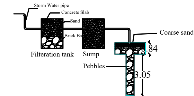
CONSTRUCTION DETAILS OF RECHARGE TRENCH
