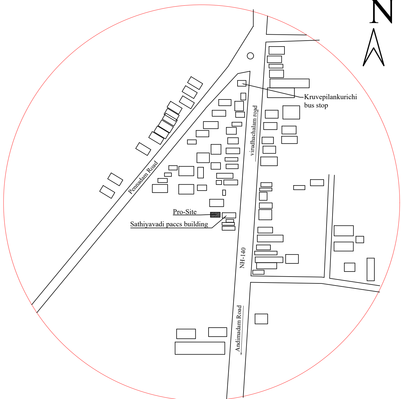
TOPO PLAN(300M R )scale 1:5000
