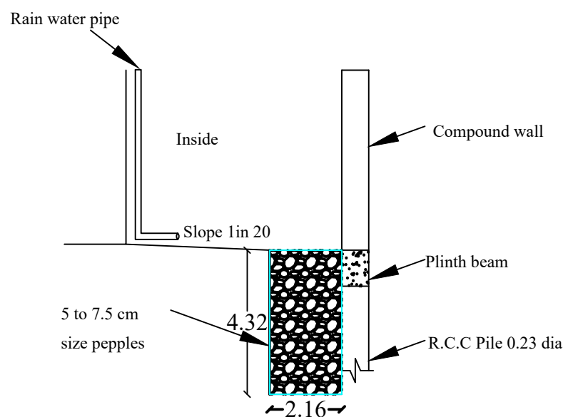
RAIN WATER COLLECTION TRENCH:- NOT TO SCALE
