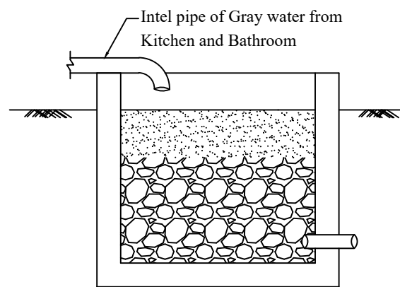
GREY WATER RECYCLING CHAMBER:-
