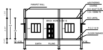
SECTION "A-B"
