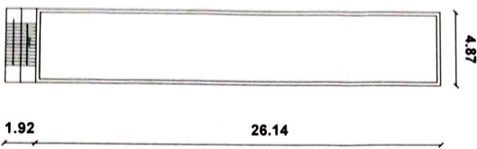
TERRACE FLOOR PLAN
