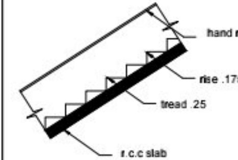
STAIR
