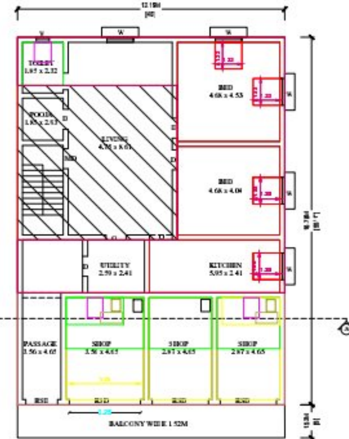
EX. AND PRO. FIRST FLOOR PLAN
