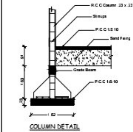
COLUMN DETAIL
