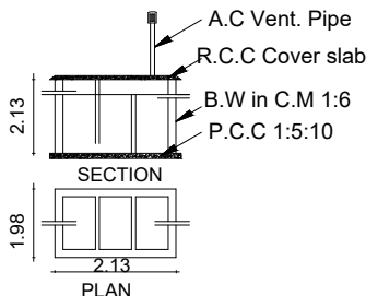
SEPTICTANK DETAILS
