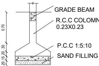
SECTION FOUNDATION DETAILS
