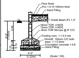
FOUNDATION DETAILS
