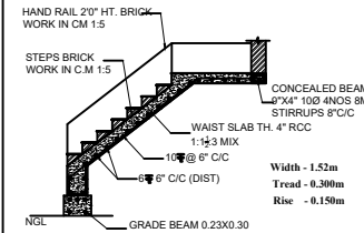
STAIRCASE DETAILS (Scale 1:50)
