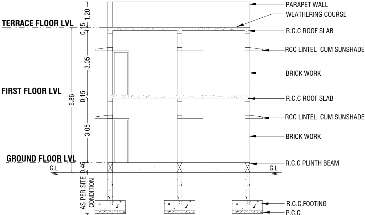
SECTION "AA" @ NORTH SIDE
