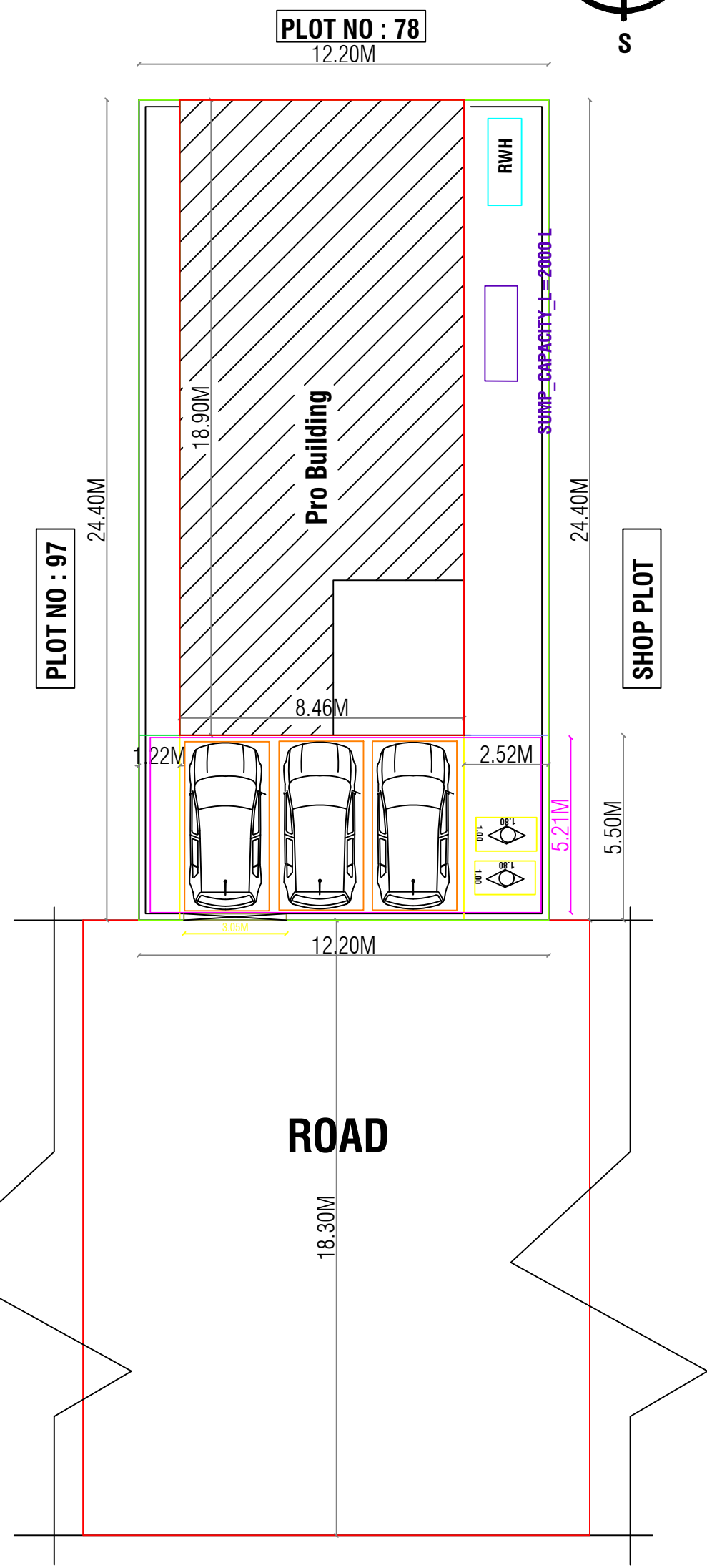
SITE PLAN
