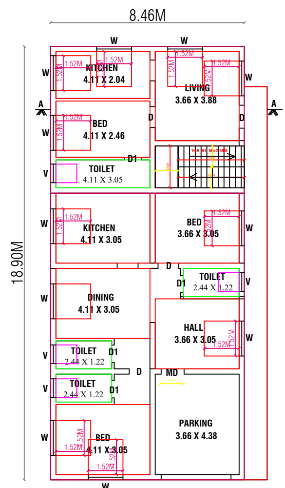
FLOOR-GROUND
