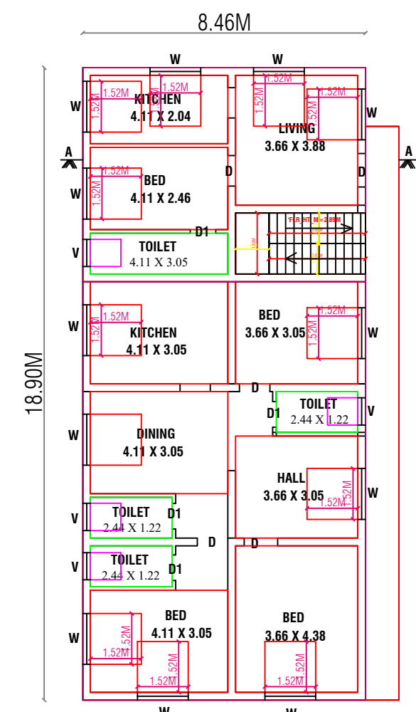
FLOOR-01
