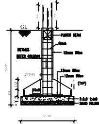
FOUNDATION DETAILS
