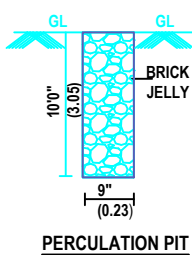
PERCOLATION PIT
