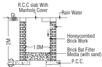
DETAILS OF RAIN WATER COLLECTION PIT
