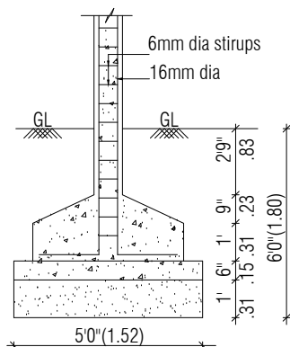
FOUNDATION DETAIL
