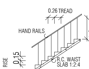
STAIRCASE DETAILS
