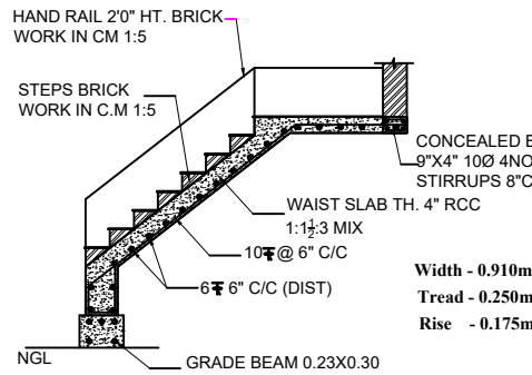
STAIRCASE DETAILS (Scale 1:50)
