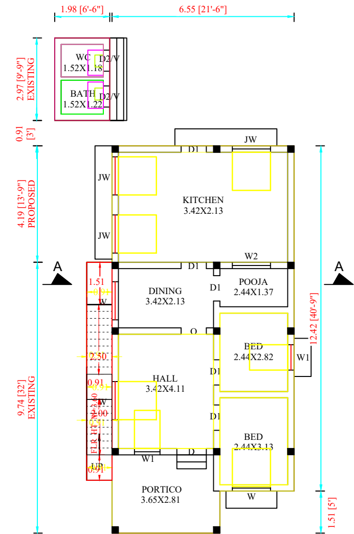
PRO. ADD. GROUND FLOOR PLAN
