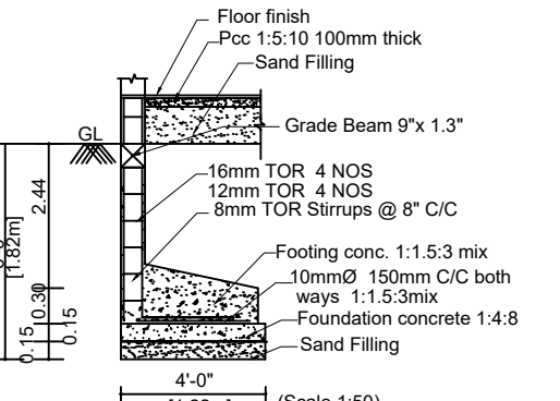
FOUNDATION DETAILS
