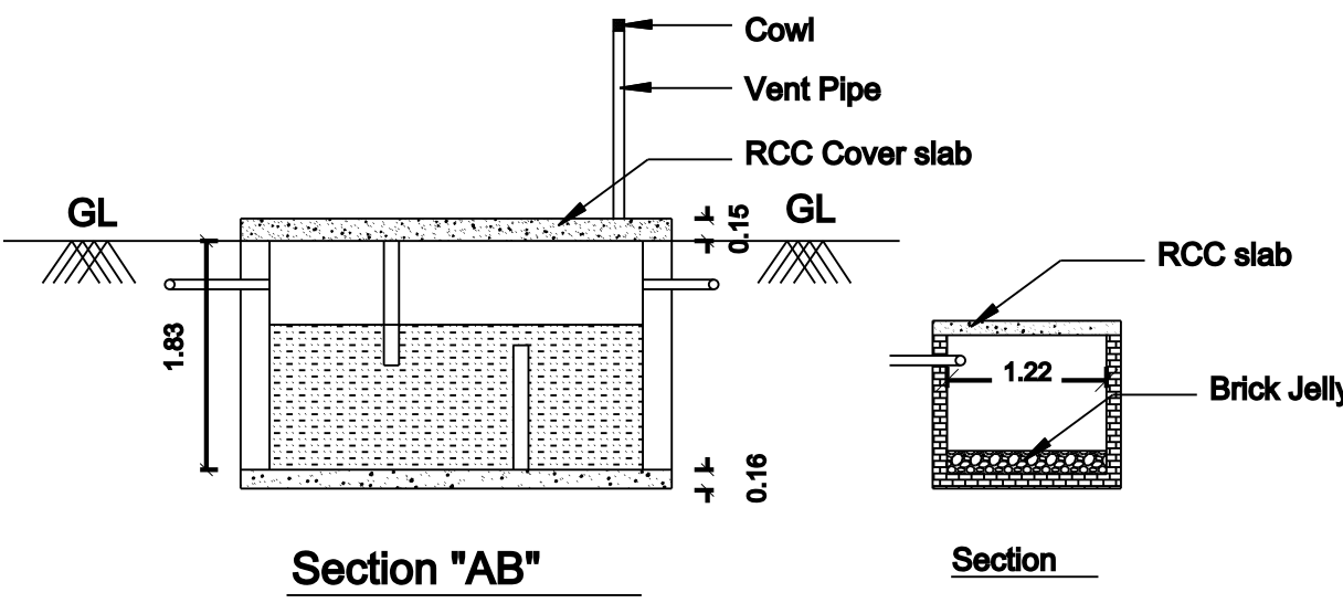
Section "AB"
