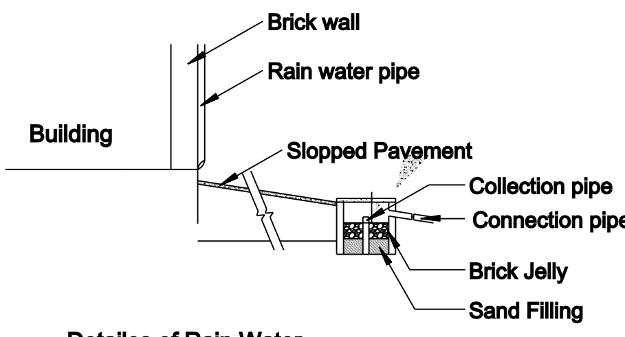
Details of Rain Water Harvesting pit
