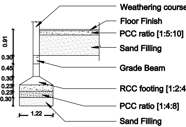
Foundation Details
