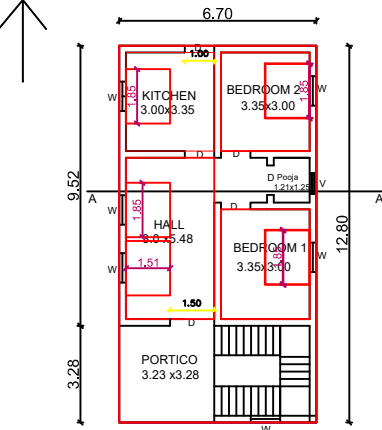
PRO. GROUND FLOOR PLAN
