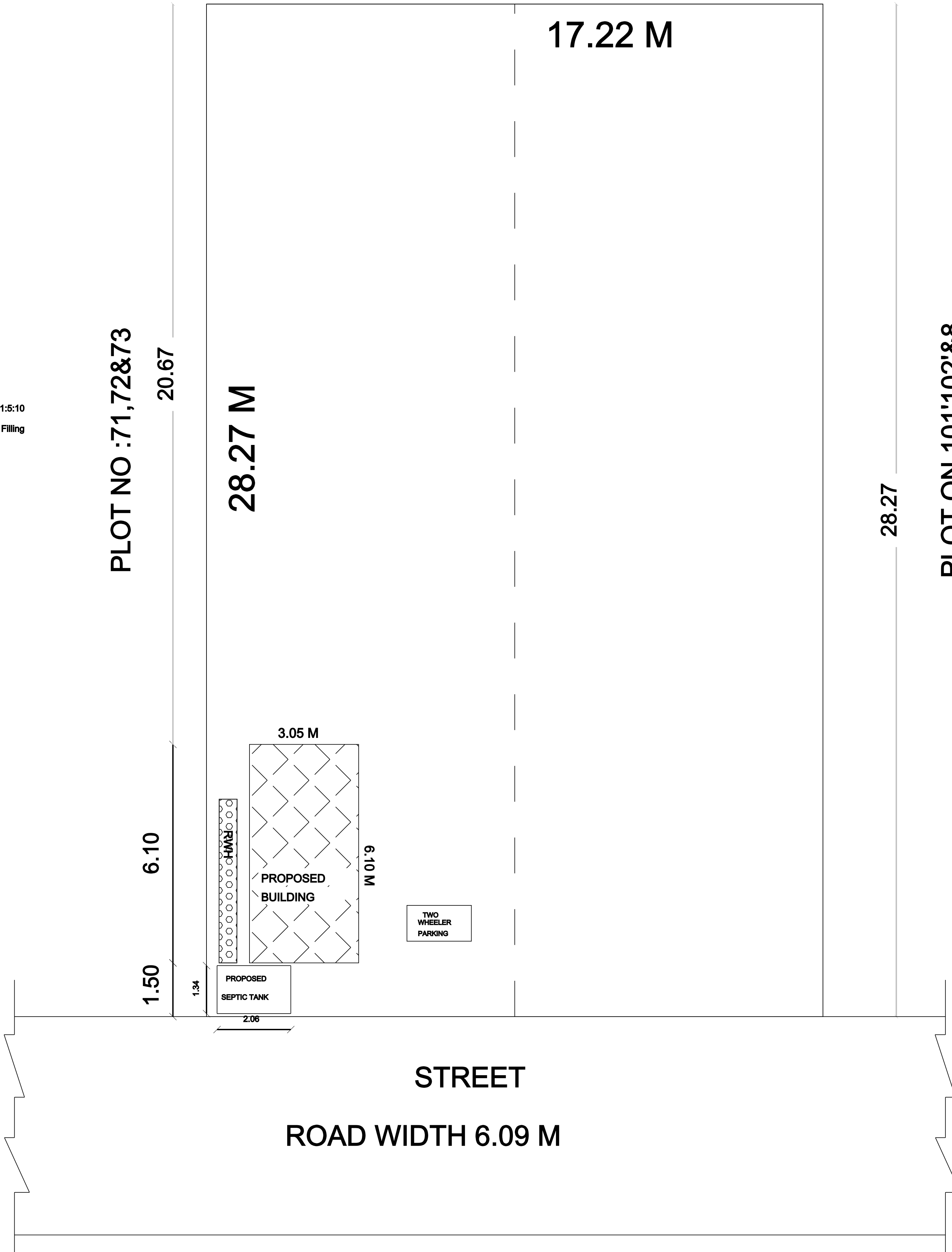
SITE PLAN
