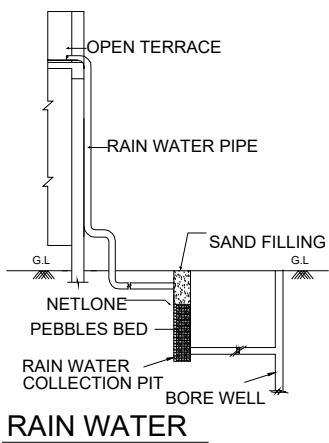
RAIN WATER
