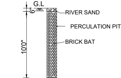
PERCULATION PIT
