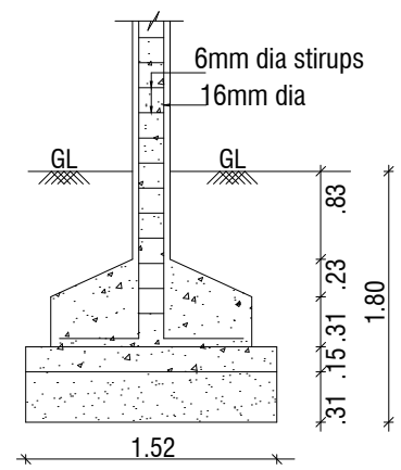
FOUNDATION DETAIL
