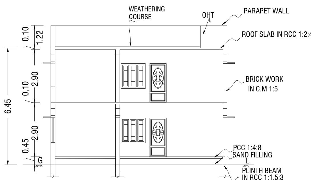
SECTION AT 'AB'
