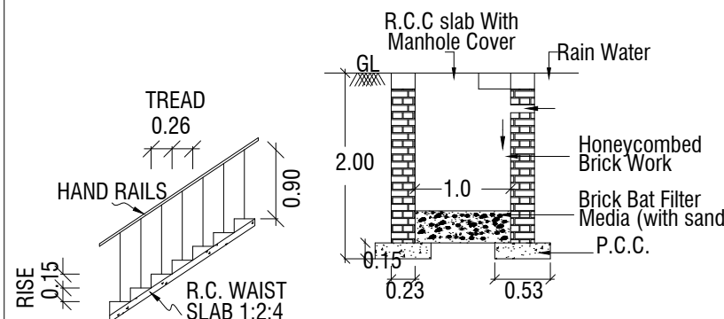
STAIRCASE DETAILS DETAILS OF RAIN WATER COLLECTION PIT SCALE:- 1"=4'0"
