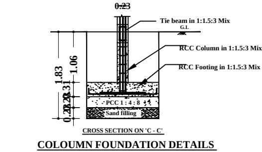
COLOUMN FOUNDATION DETAILS
