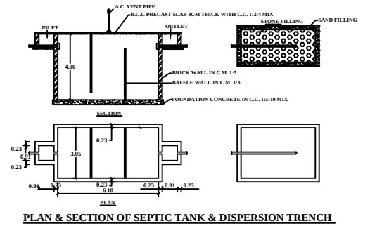
PLAN & SECTION OF SEPTIC TANK & DISPERSION TRENCH
