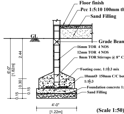
FOUNDATION DETAILS
