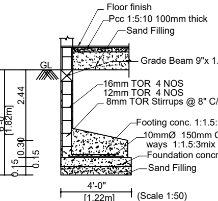
FOUNDATION DETAILS
