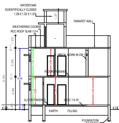
SECTION "A-B"
