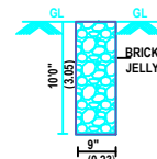
PERCULATION PIT
