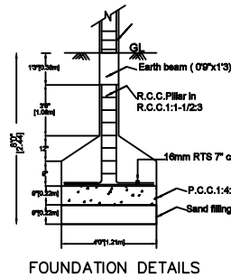
FOUNDATION DETAILS
