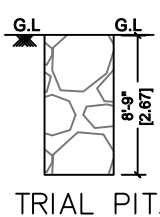
TRIAL PIT
