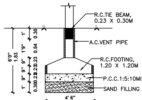
FOUNDATION DETAILS
