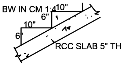
STAIR DETAIL
