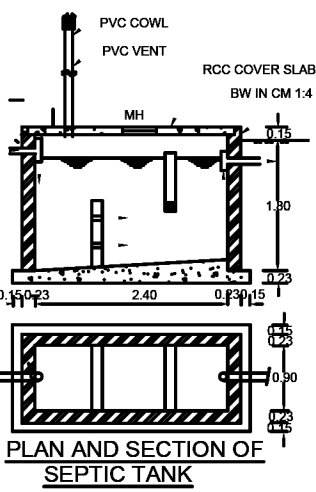
PLAN AND SECTION OF SEPTIC TANK
