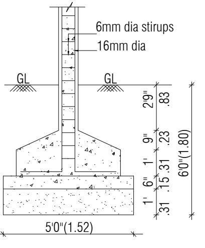
FOUNDATION DETAIL
