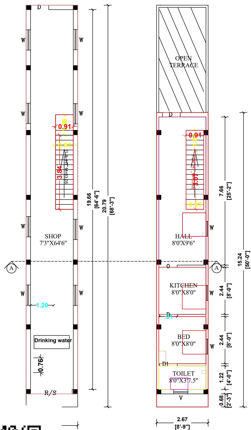
FLOOR PLAN PROPOSED FIRST FLOOR PLAN
