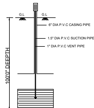
BORE WELL
