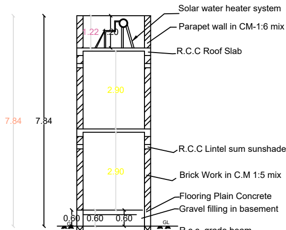
SECTION ON - "XX"
