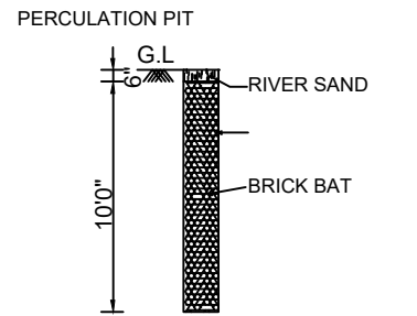
PERCOLATION PIT
