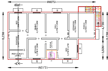
EXISTING GROUND FLOOR PLAN
