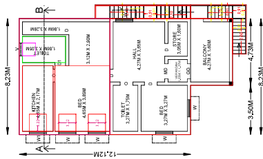
EXIST FIRST & PRO FIRST FLOOR PLAN
