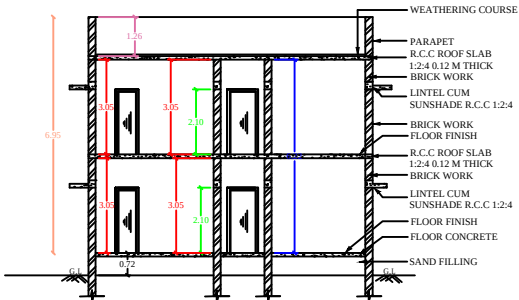
SECTION "N-R"
