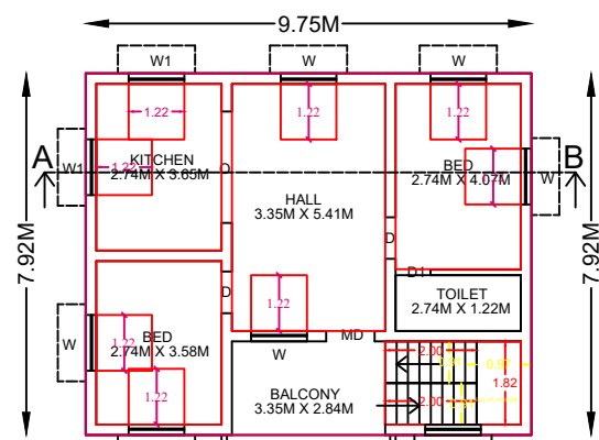
TYPICAL FIRST & SECOND FLOOR PLAN
