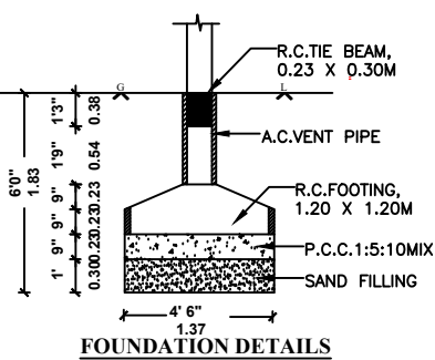
FOUNDATION DETAILS
