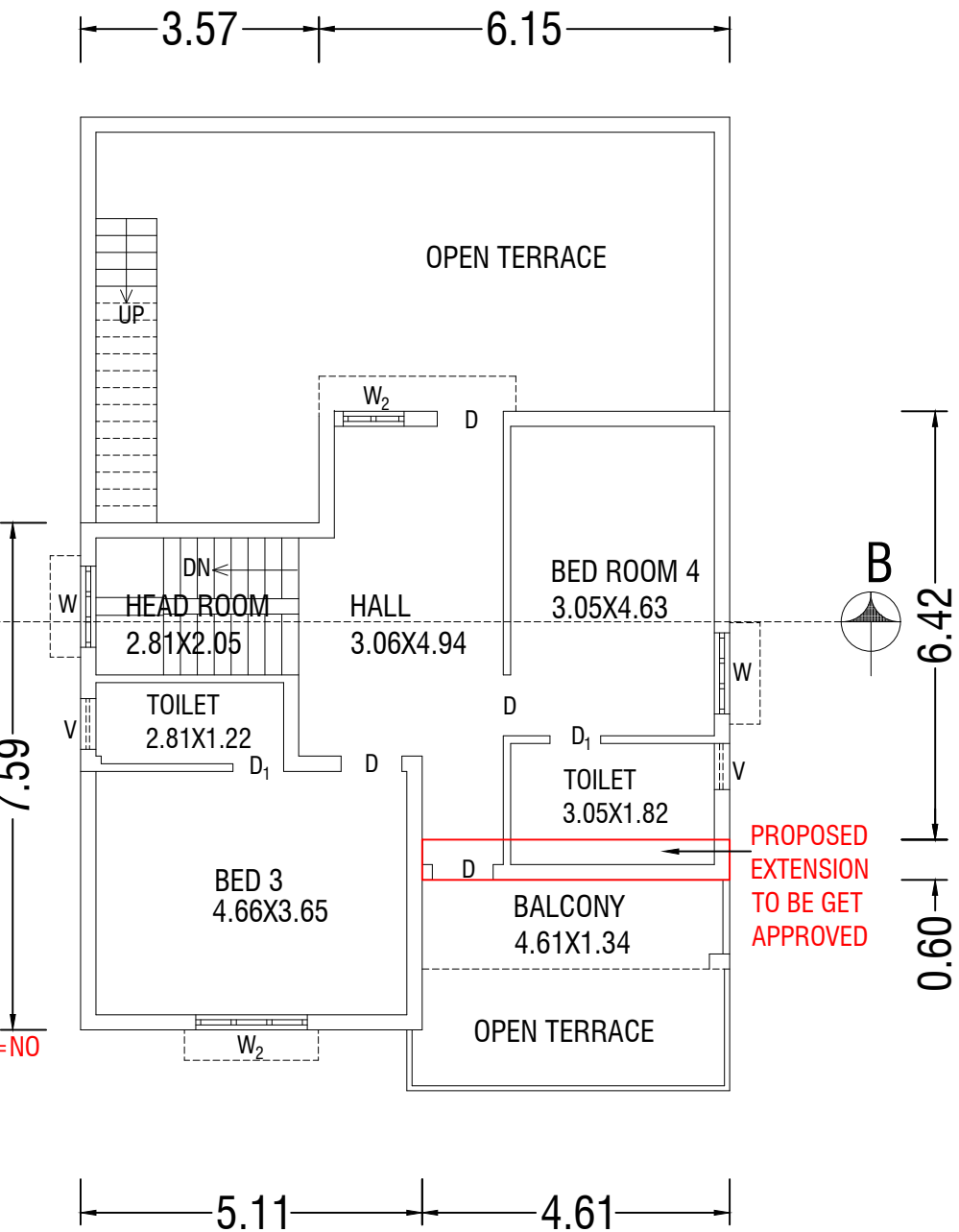
APPROVED FIRST FLOOR PLAN & PROPOSED ADDITIONAL FIRST FLOOR PLAN
