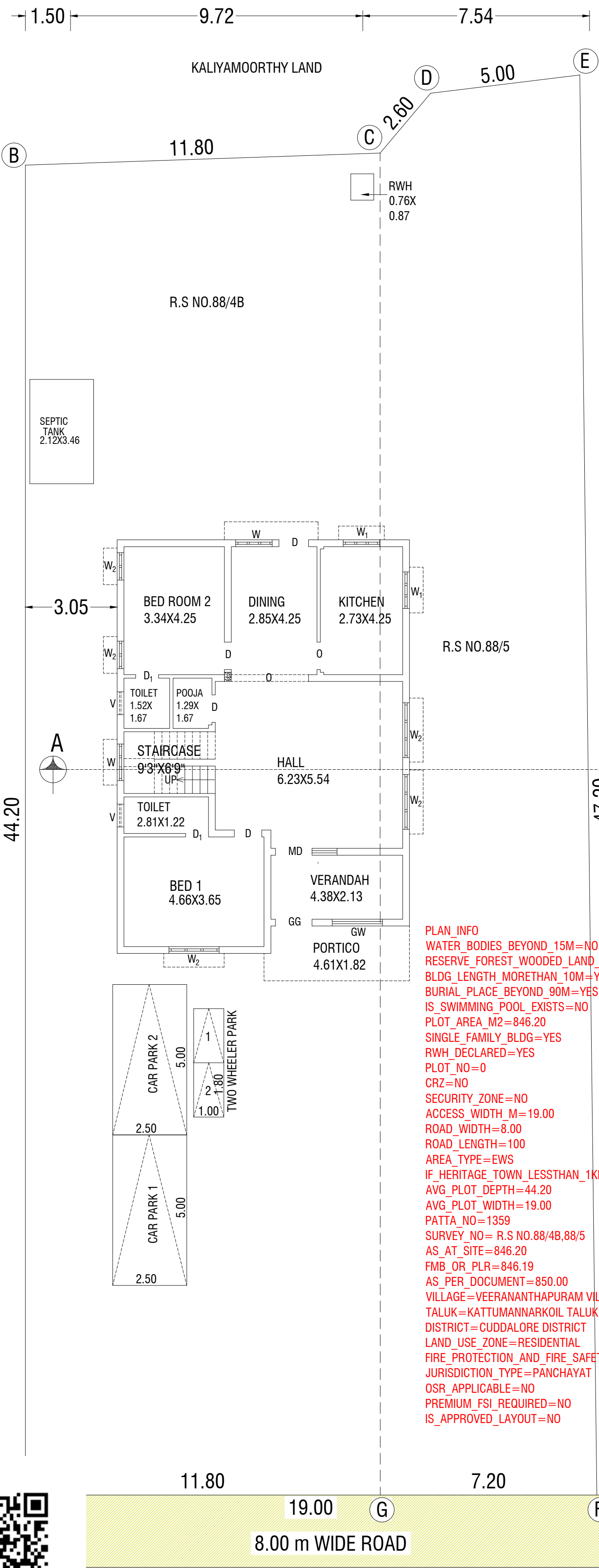
CUM APPROVED GROUND FLOOR PLAN
