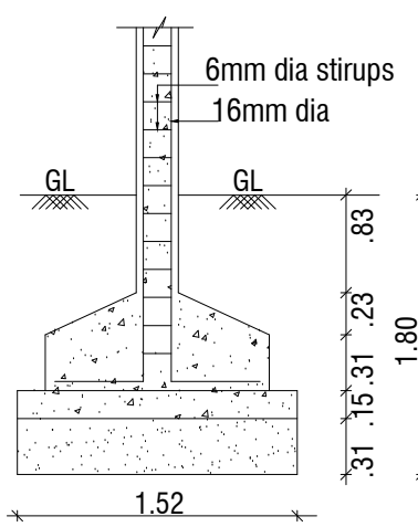
FOUNDATION DETAIL SCALE (1:50)
