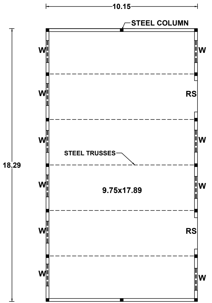
PLAN OF COMMERCIAL BUILDING
