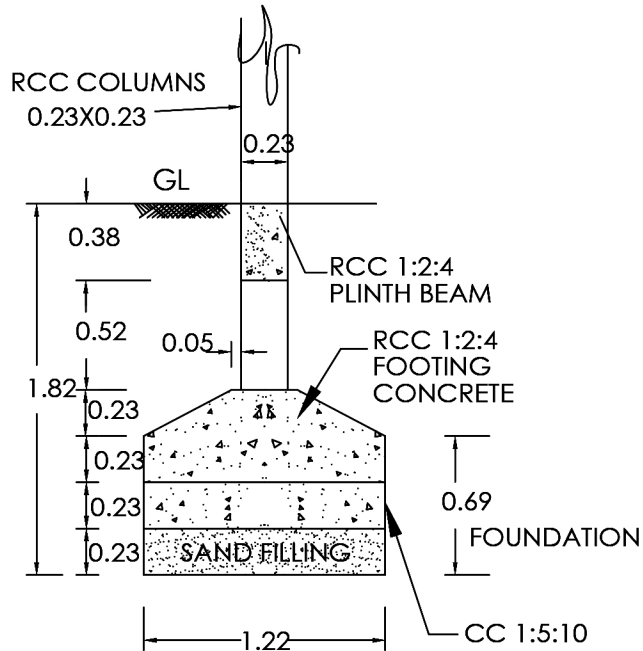
FOUNDATION DETAILS
