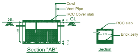
Section "AB"
