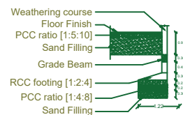
Foundation Details
