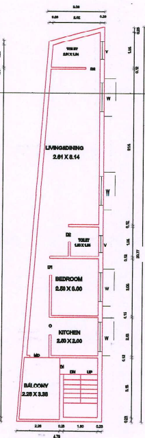
Second Floor Plan Floor02 (Proposed)
