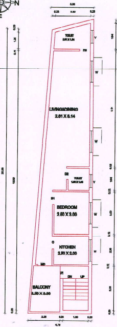
First Floor Plan Floor01 (Proposed)
