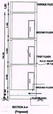
SECTION A-A (Proposed)
