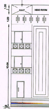
ELEVATION (Proposed)
