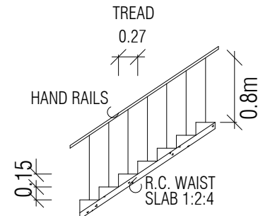
STAIRCASE DETAILS
