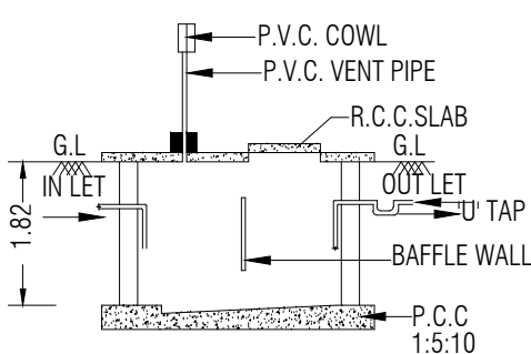
SEC. OF SEPTIC TANK"AA" PLAN OF SEPTIC TANK
