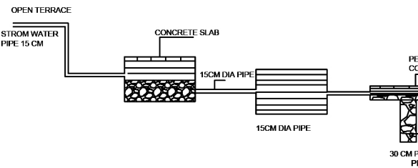
RAIN WATER HARVESTING SYSTEM
