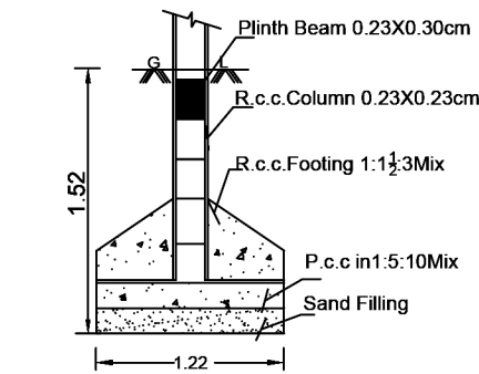
"FOUNDATION DETAILS"
