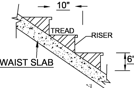
" STAIRCASE DETAIL(NTS)"
