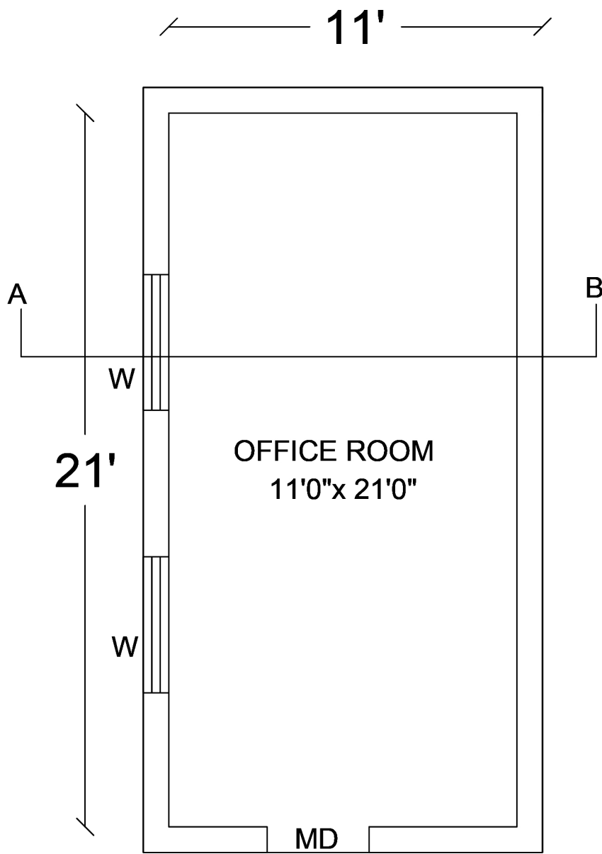
PLAN
