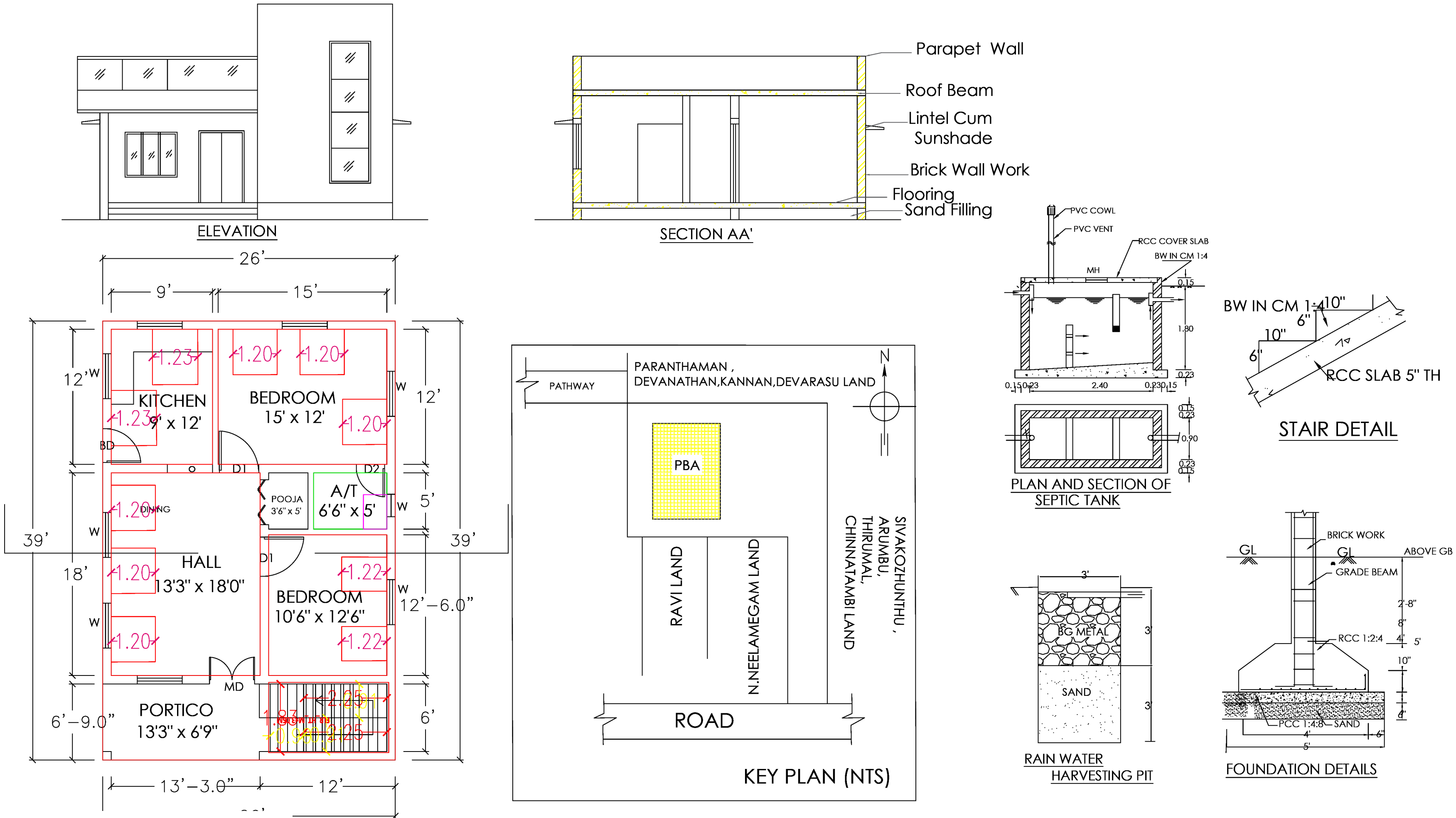
PLAN
