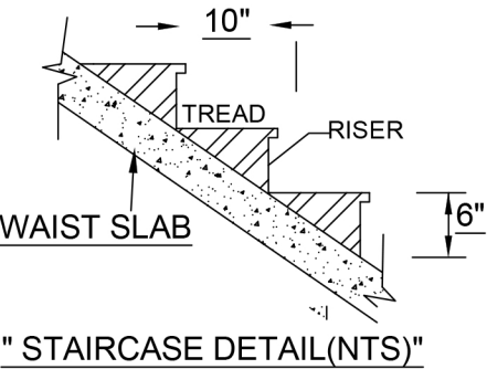
" STAIRCASE DETAIL(NTS)"
