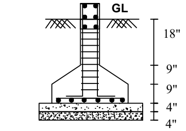
FOUNDATION DETAILS
