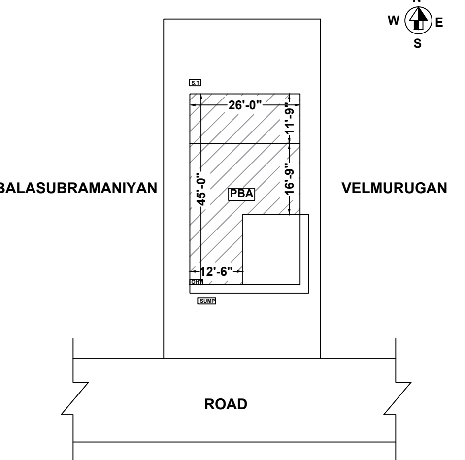
SITE PLAN
