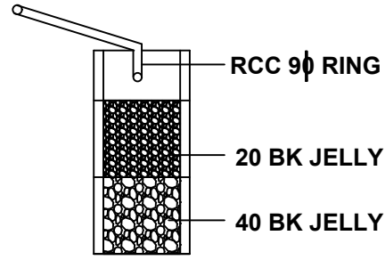
RAINWATER HARVEST PIT
