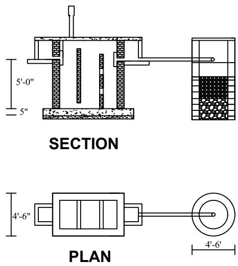
SEPTIC TANK & SOAK PIT
