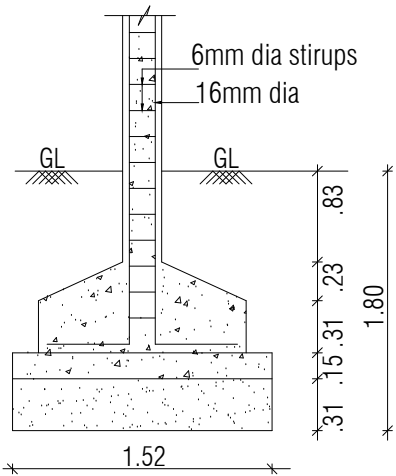
FOUNDATION DETAIL
