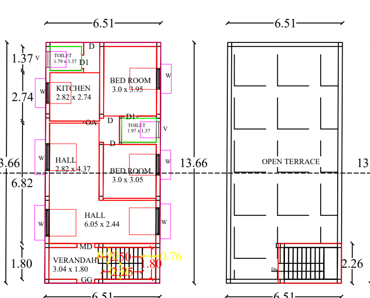
BLOCK-2 GROUND FLOOR PLAN BLOCK-2 TERRACE FLOOR PLAN
