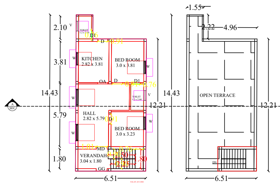
BLOCK-1 GROUND FLOOR PLAN BLOCK-1 TERRACE FLOOR PLAN
