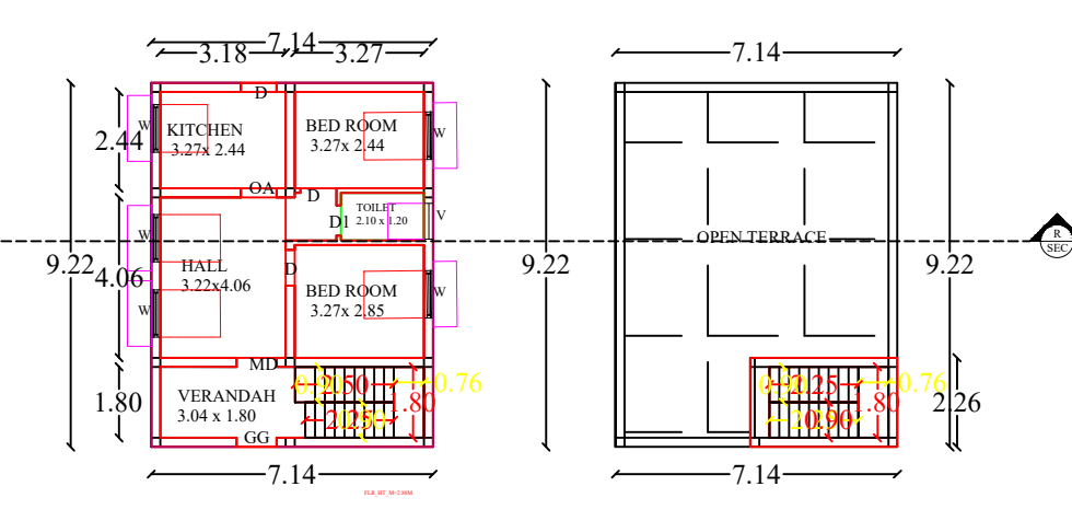
BLOCK-3 GROUND FLOOR PLAN BLOCK-3 TERRACE FLOOR PLAN
