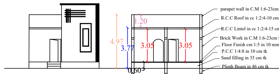
FRONT ELEVATION SECTION ON "AR"
