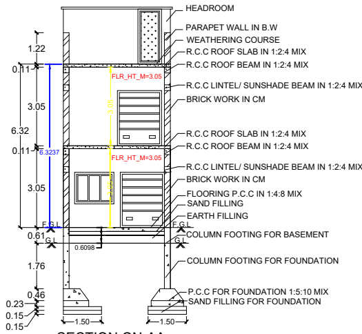
SECTION ON-AA
