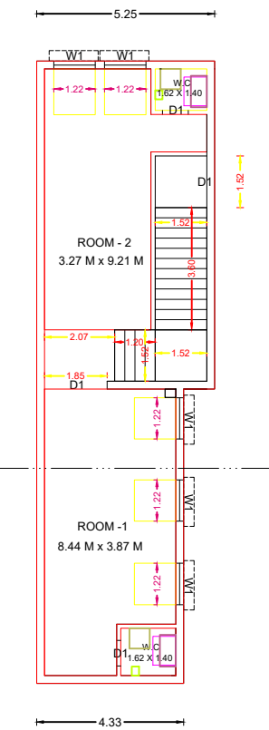
PRO.FIRST FLOOR PLAN
