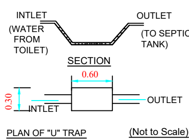
PLAN OF "U" TRAP (Not to Scale)
